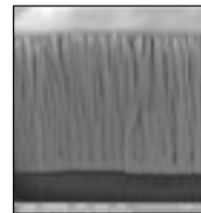
Tantalum on Nitinol (cross-section)
