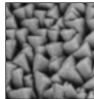
Tantalum on PEEK (from above)
